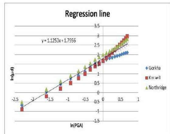
Figure 11: Regression analysis of Time History Results for trapezoidal deck bridge pier
