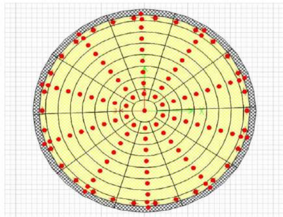
Figure 2: Fiber distribution in cross section of pier
