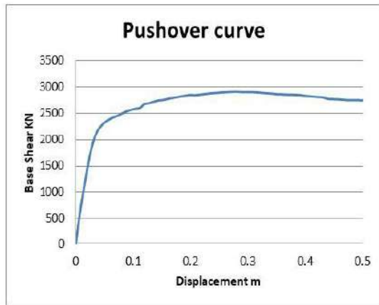
Figure 9: Push over curve for rectangular section
