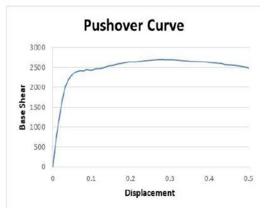
Figure 8: Push over curve for trapezoidal section
