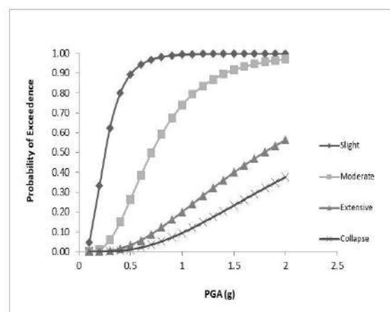
Figure 12: Fragility curve for rectangular deck section pier
