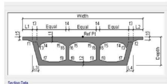
Figure 1: Typical section detail of Trapezoidal box girder
