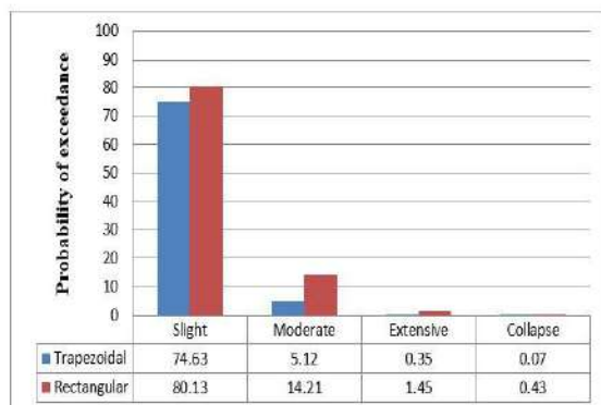
Figure 14: Probability of exceedance for design basis earthquake
