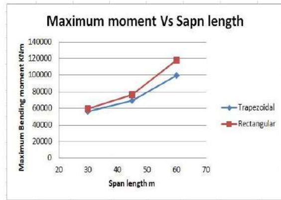
Figure 5: Maximum Bending moment of different span length
