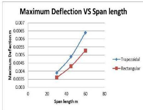
Figure 7: Maximum Deflection of top flange for different span length
