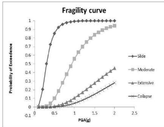
Figure 13: Fragility curve for Trapezoidal deck section pier
