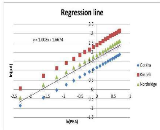
Figure 10: Regression analysis of Time History Results for Rectangular deck bridge pier
