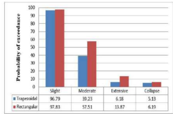
Figure 15: Probability of exceedance for Maximum Considered Earthquake
