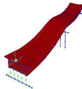
Figure 4: Deformed shape of trapezoidal and rectangular box girder model
